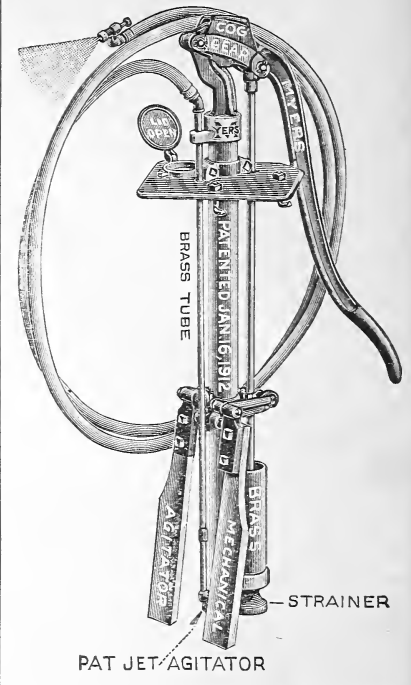
Barrel Spray Pump
